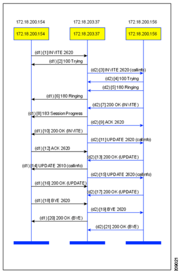
Figure 9 Sample GDVE to GSSRS call with Secure Audio and Nonsecure Video
